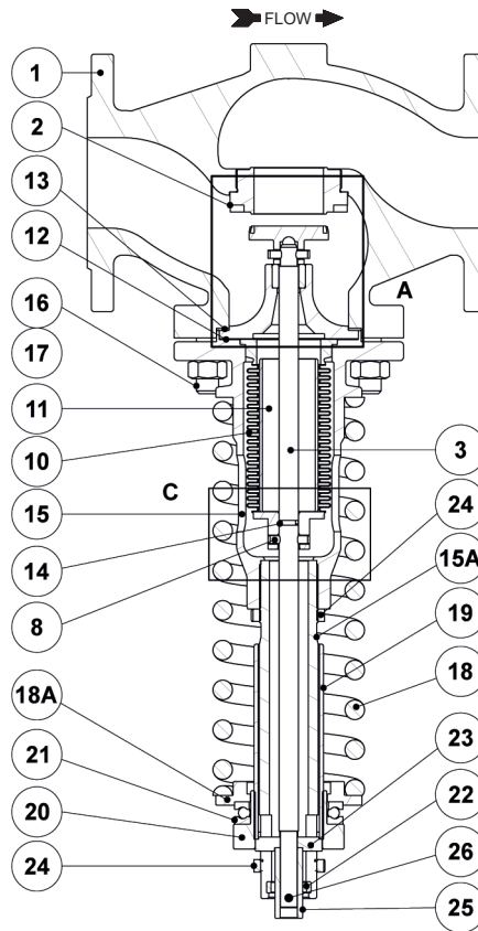
DN 65 to DN 100
