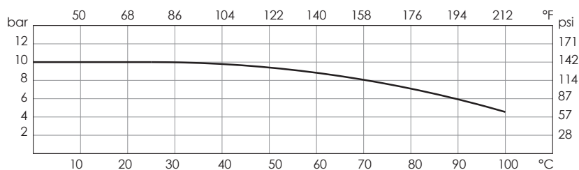
Druck-/Temperatur Diagramm / Pressure/temperature chart
